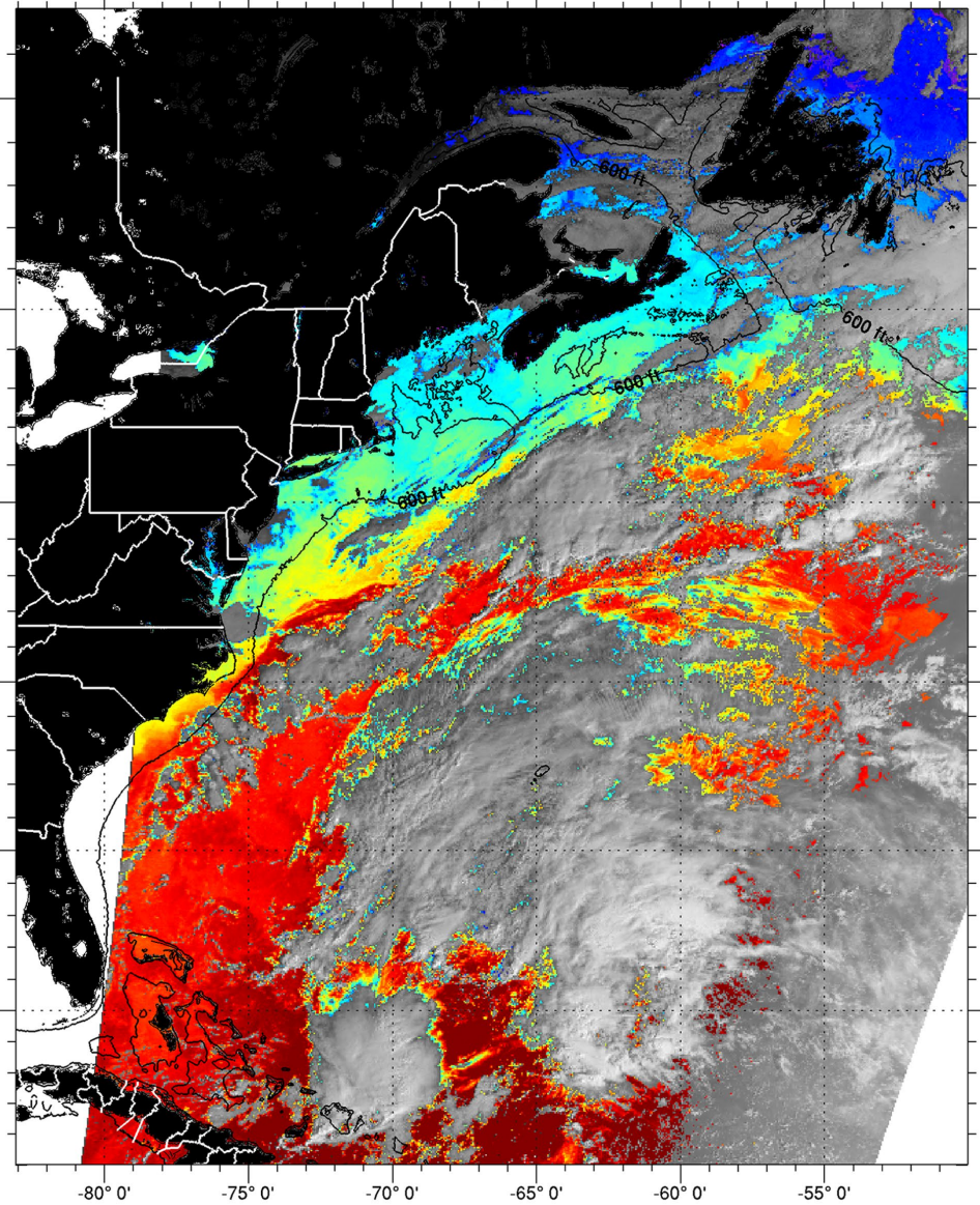
RU COOL NOAA-12 Sea Surface Temperature: October 29, 1992 1211 GMT
