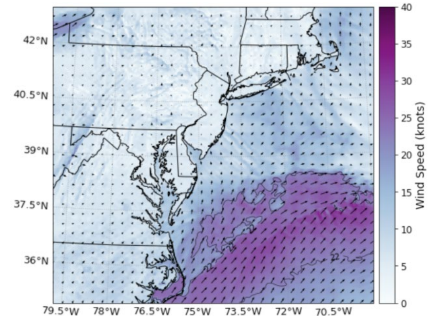
RUWRF Weather Model
